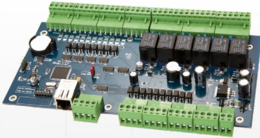
Access Control Panel ACP2000A
